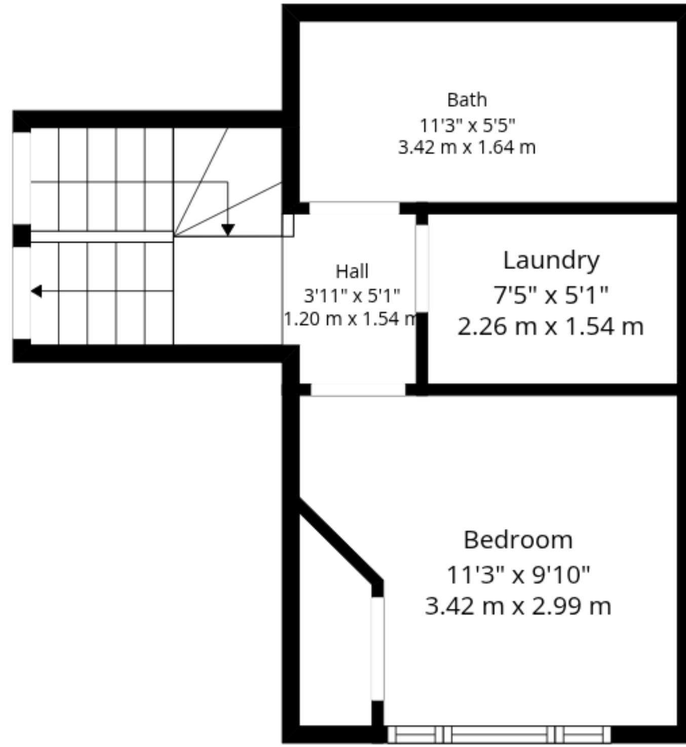
4th Floor
