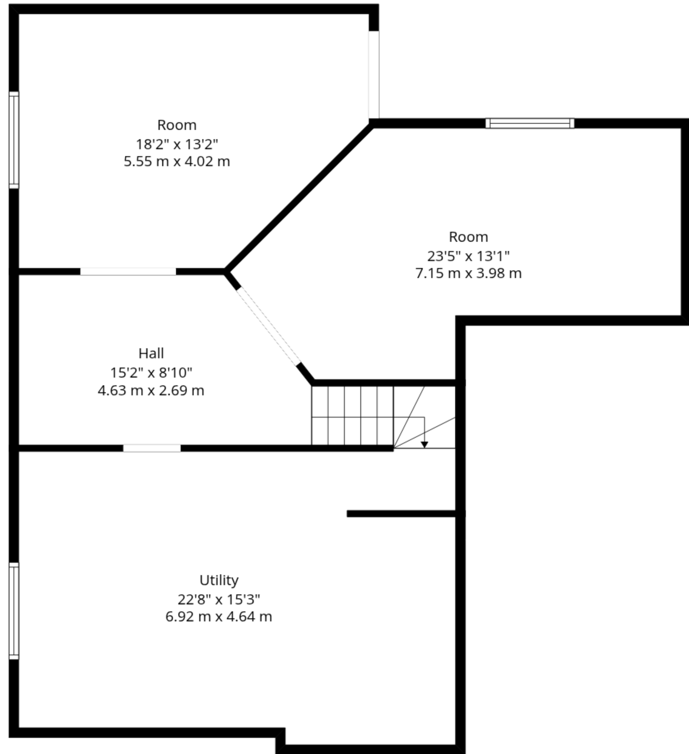
1st Floor
